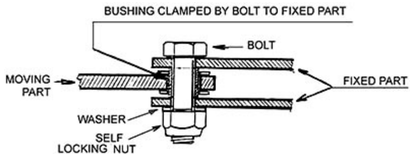
DWG 4-13A Tail Bearing System Parts
