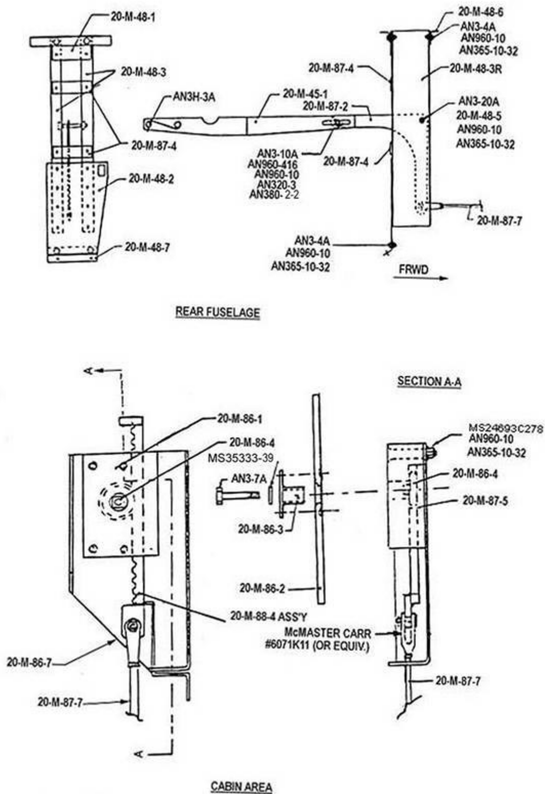
DWG 8-19 Trim System Parts
