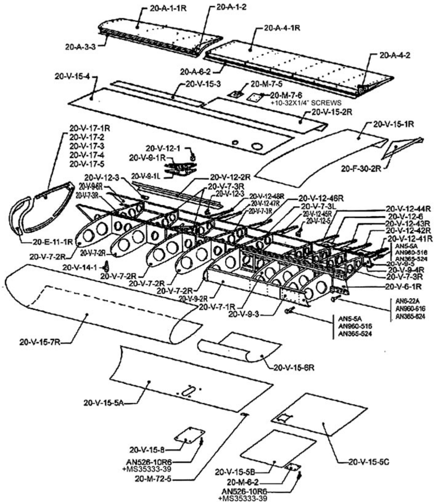
DWG 1-2 Wing Parts
